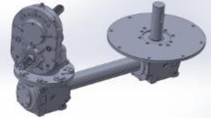
Full PTO Gearbox Drive Render
