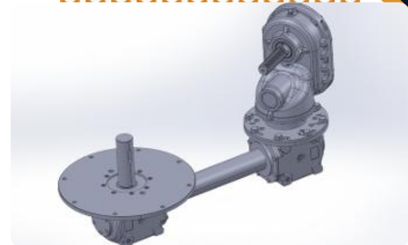
Full PTO Gearbox Drive Render
